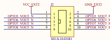
OUTPUT CONNECTOR
