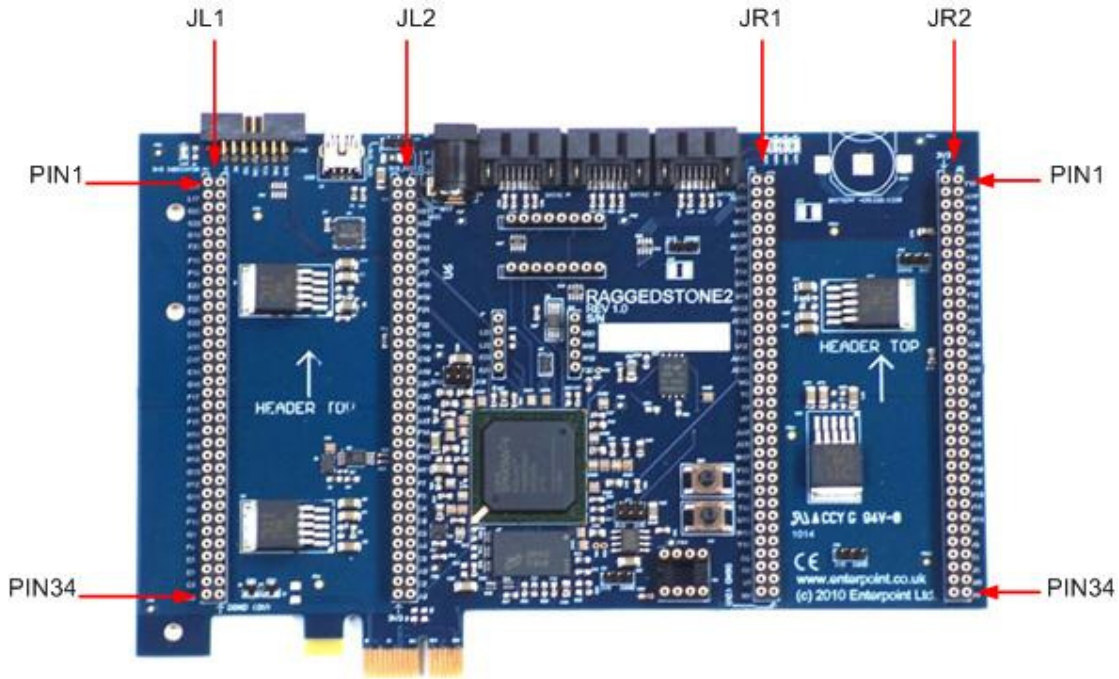
Figure 7 – Raggedstone2 DIL Headers
